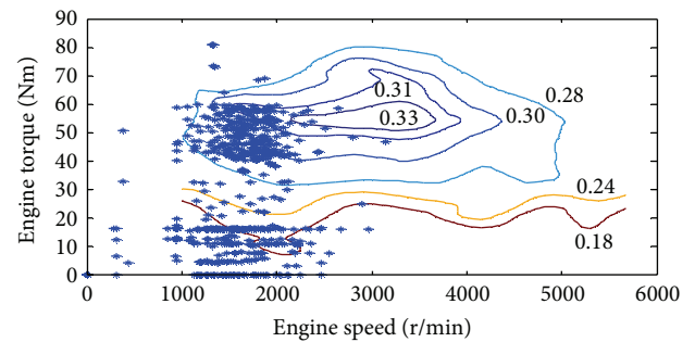
FIGURE 8: Engine operating points of strategy 1.
