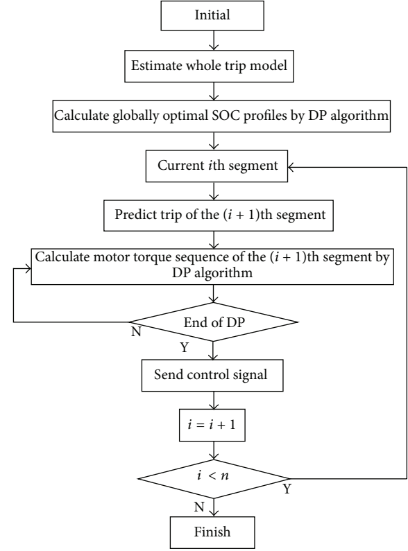
FIGURE 1: Flow chart of trip-based EMS.
