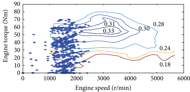
FIGURE 9: Engine operating points of strategy 2.
